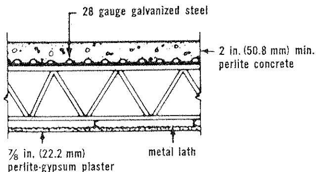
Typical lightweight perlite insulating concrete roofdeck design with 3 hour fire rating. (Underwriters' Laboratories Class C-3, Design No. P407)
